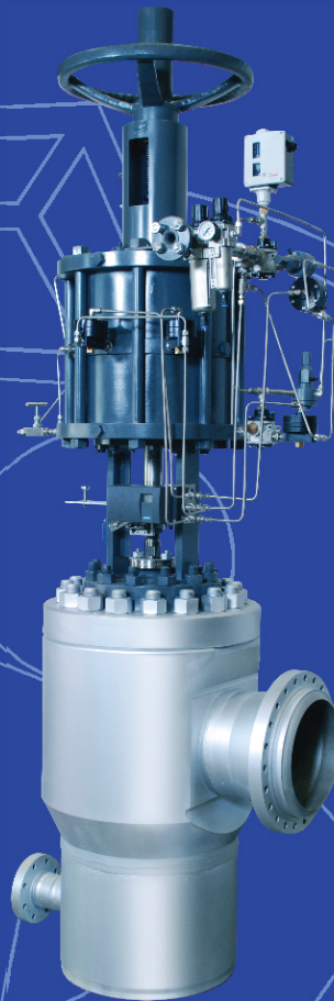
HP Bypass valve for combined cycle power plant
