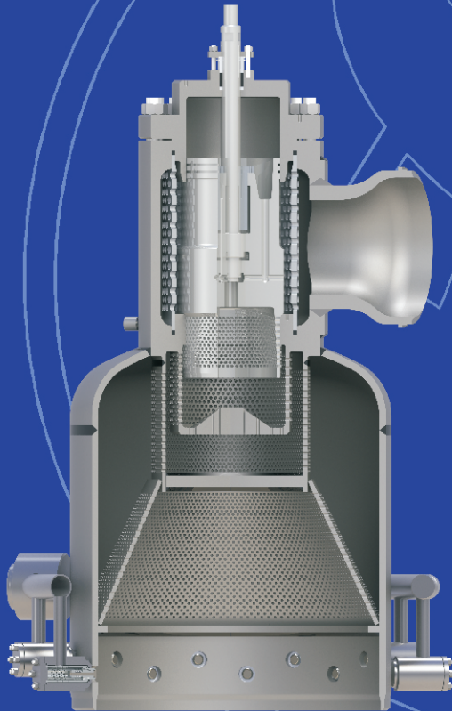
LP Bypass valve for 660 MW power plant
