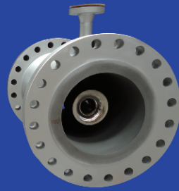
Venturi desuperheater
