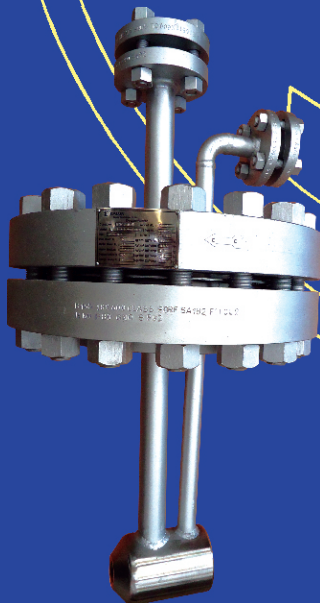
Steam laval jet atomizing desuperheater
