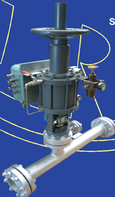
Desuperheater-integral multinozzle type
