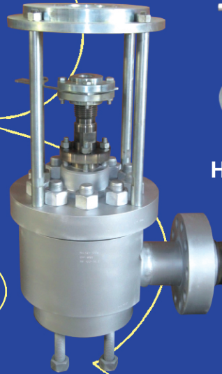
Spray water control valve for 660 mw
